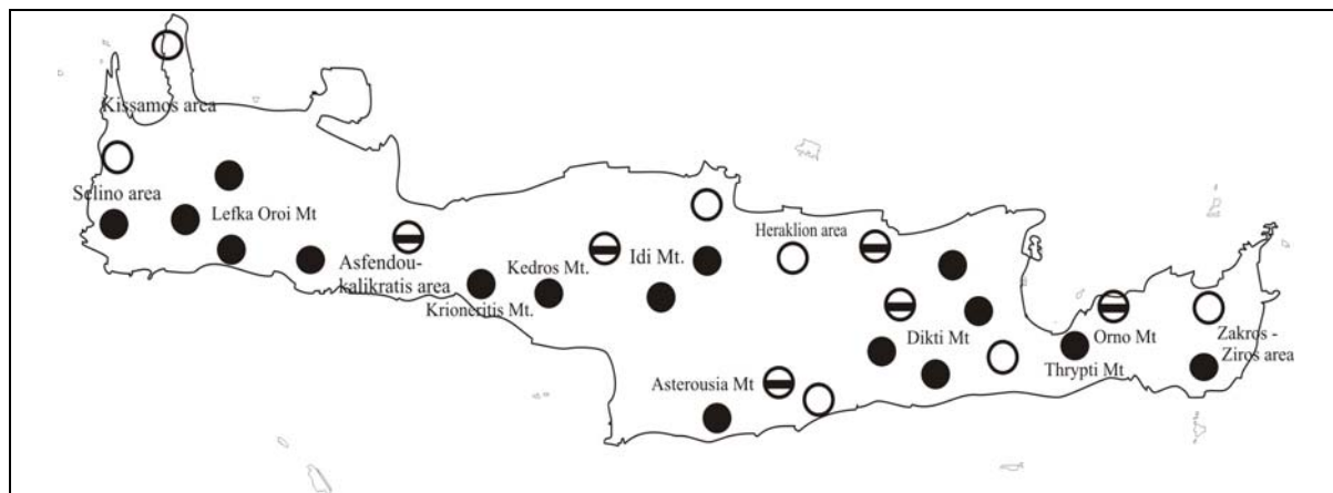
Figure 1. Golden Eagle territories in Crete
